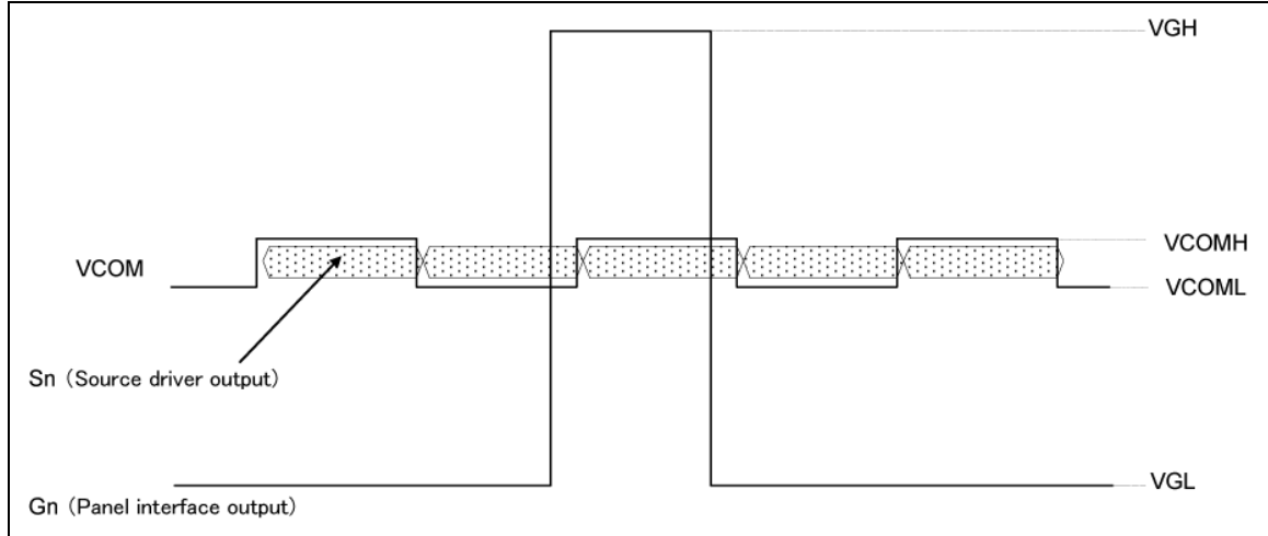
Figure 66 Voltage Application to TFT Display
